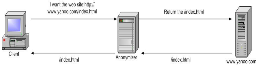
Figure 1 Anonymizer
